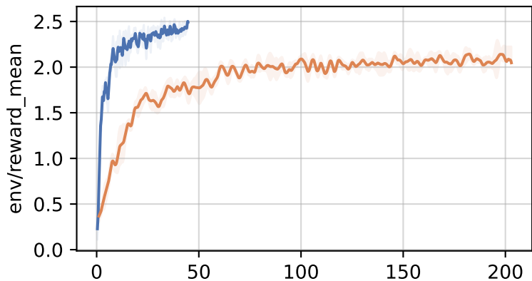
sentiment-analysis:lvwerra/distilbert-imdb
