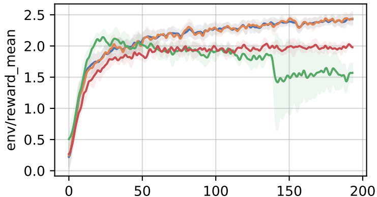
sentiment-analysis:lvwerra/distilbert-imdb
