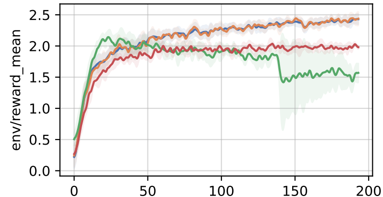
sentiment-analysis:lvwerra/distilbert-imdb
