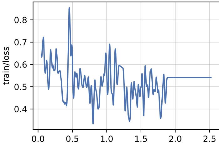
models/rm/rm_descriptiveness_1b
