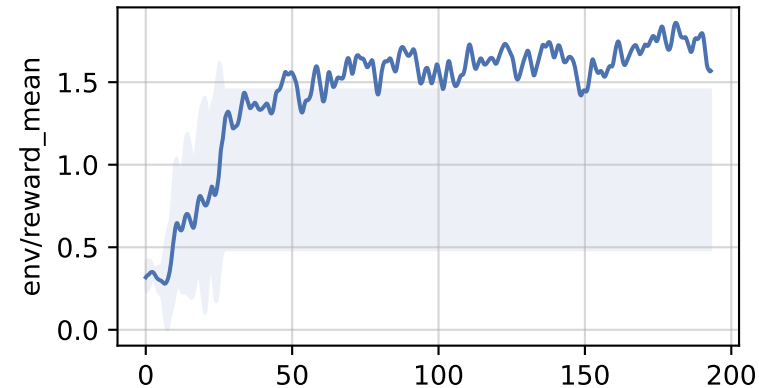
sentiment-analysis:lvwerra/distilbert-imdb
